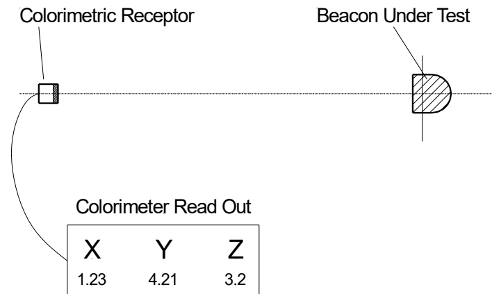
Figure 40 Standard arrangement
