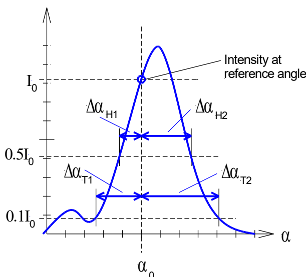
Figure 29 Asymmetrical Intensity Distribution showing Reduced Values
