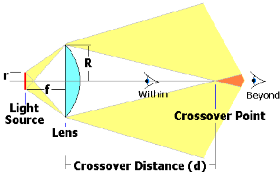
Figure 25 Crossover Distance
