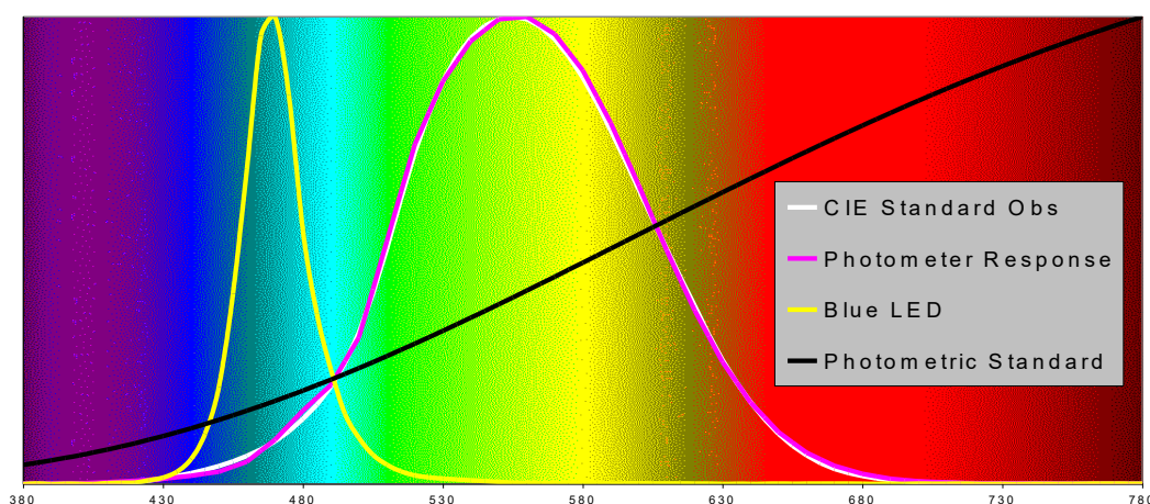
Figure 3 Spectral Plot showing Differences between Typical Photometer Response and V(\lambda)
