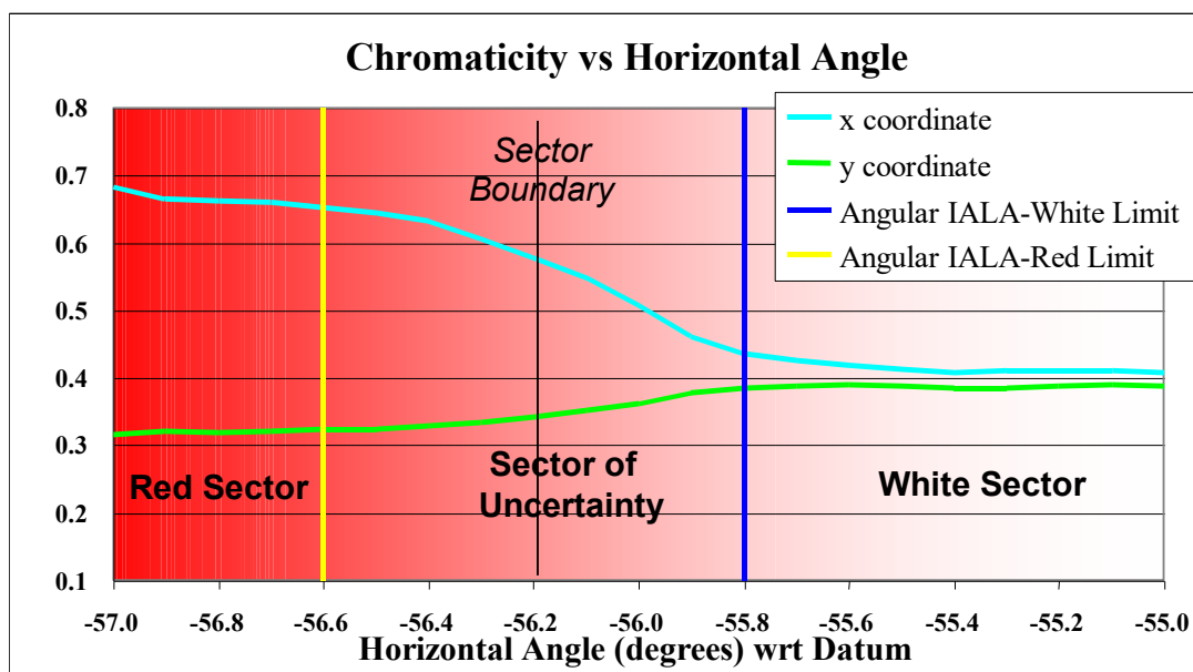
Figure 31 Plot of chromaticity across the boundary between red and white sectors
